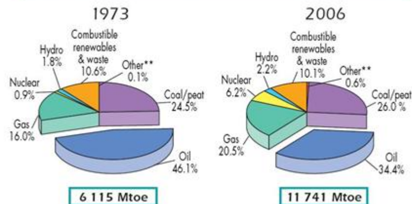
1973 and 2006 fuel shares of TPES*
